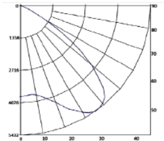
Above: Polar Candela Graph (120° Lens)
