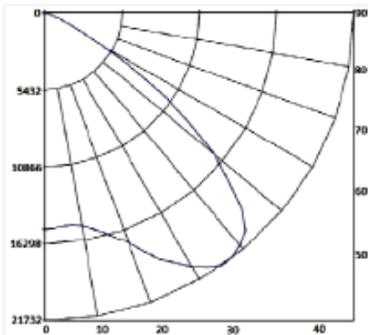
Above: Polar Candela Graph (120° Lens)
