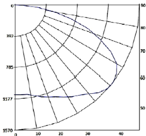
Above: Polar Candela Graph (160° Lens)
